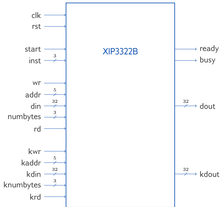
Figure 2: External interfaces of XIP3322B
