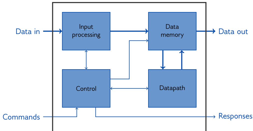
Figure 1: Internal high-level block diagram of XIP3030C
