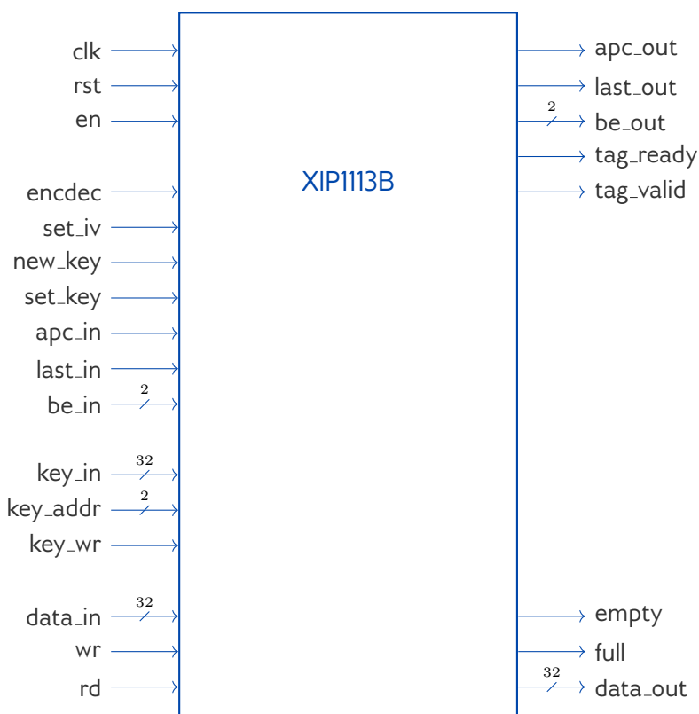
Figure 2: External interfaces of XIP1113B
